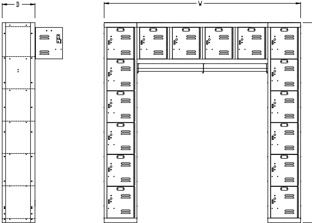
FRONT VIEW
