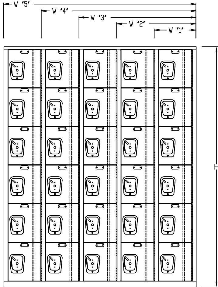
FRONT VIEW
