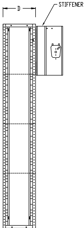
SIDE VIEW
