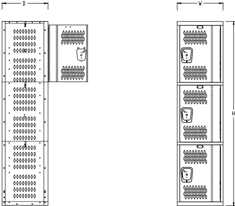
SIDE VIEW
