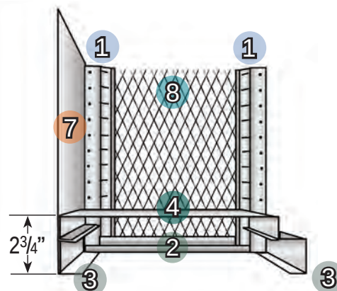
SUPERIOR® fully-framed locker bottoms are a full 2-3/4" above finished floor eliminating the need for and additional base
