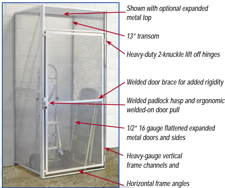
Single Tier Starter Unit
